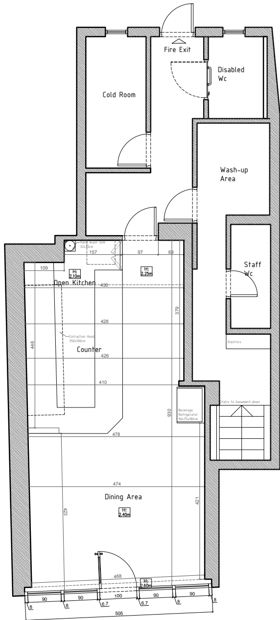
1 EXISTING LAYOUT 1/100
